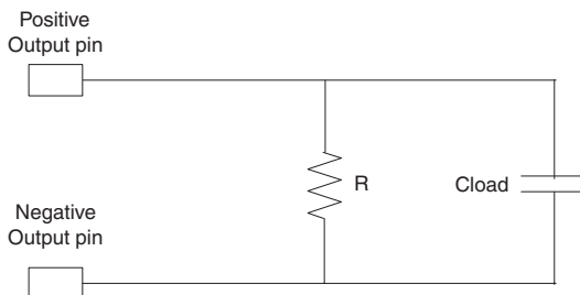
Figure 38. AC Test Conditions for the LVDS I/O Standard
