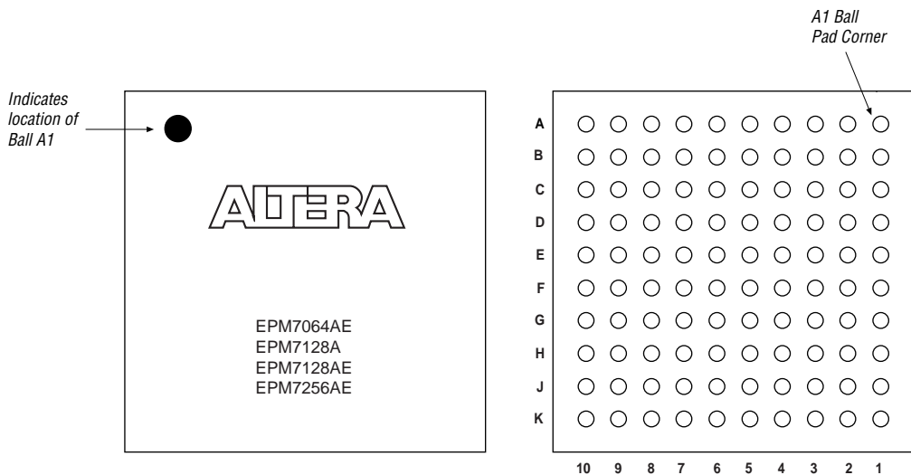
Package outline not drawn to scale.
