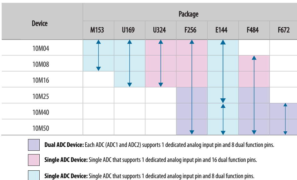
Figure 3. ADC Vertical Migration Across Intel MAX 10 Devices
