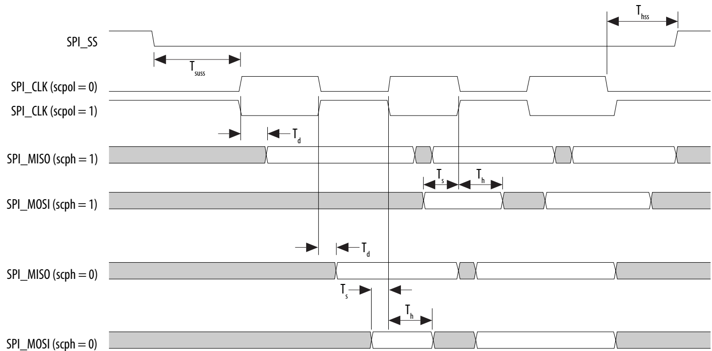
Figure 1-10: SPI Slave Timing Diagram
