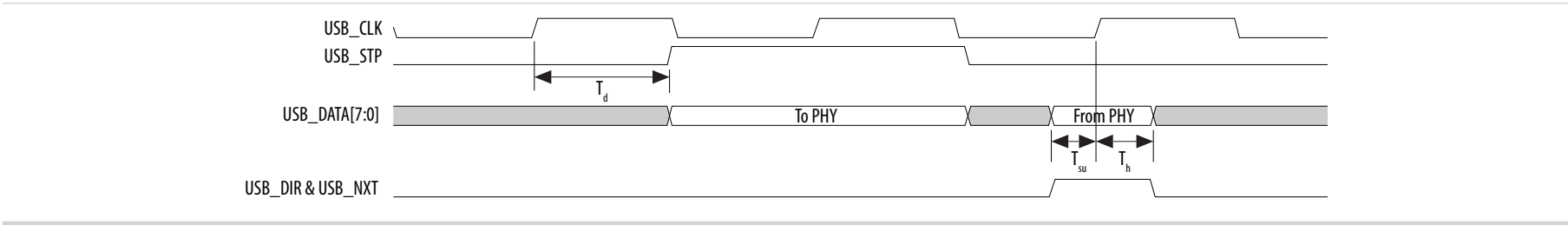
Figure 1-12: USB Timing Diagram
