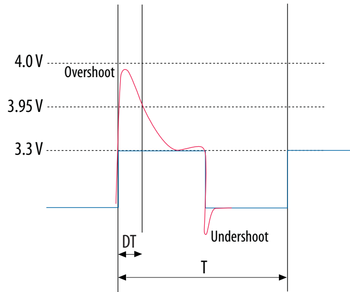
Figure 1. Stratix V Device Overshoot Duration
