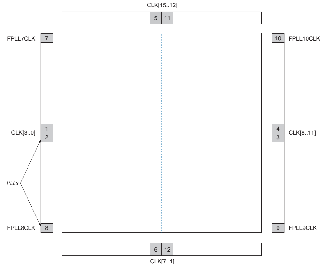
Figure 2–49. PLL Locations
