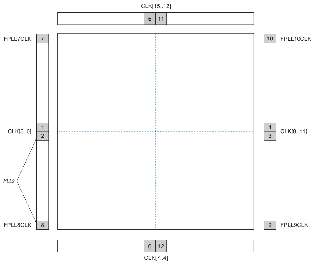
Figure 2–49. PLL Locations
