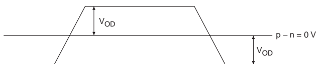
Differential Waveform
