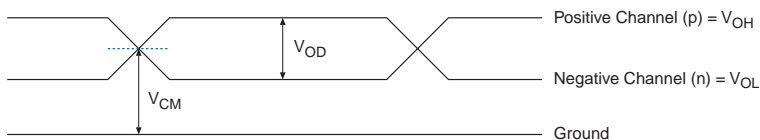
Single-Ended Waveform
