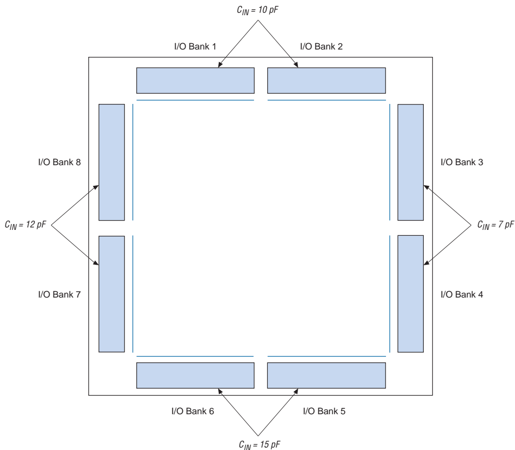
Figure 40. APEX II Maximum Input &amp; Output Pin Capacitance
