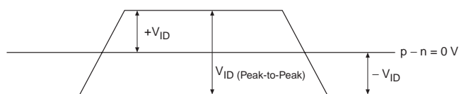
Figure 39. Transmitter Output Waveforms for Differential I/O Standards
