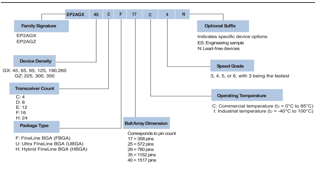
Figure 1-3. Packaging Ordering Information for Arria II Devices
