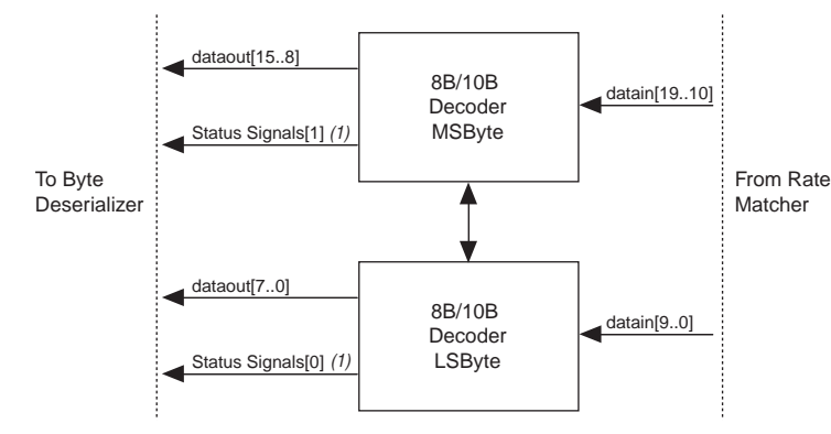
Figure 2–21. 8B/10B Decoder
