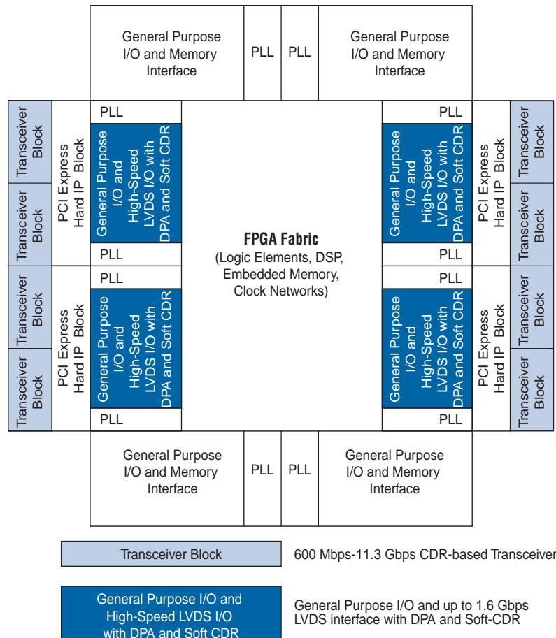
Figure 1-3. Stratix IV GT Chip View (Note 1)
