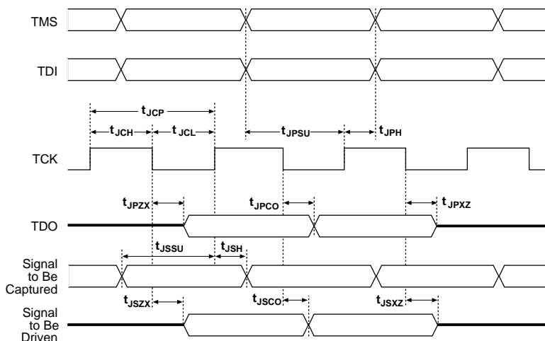
Figure 18. JTAG Waveforms
