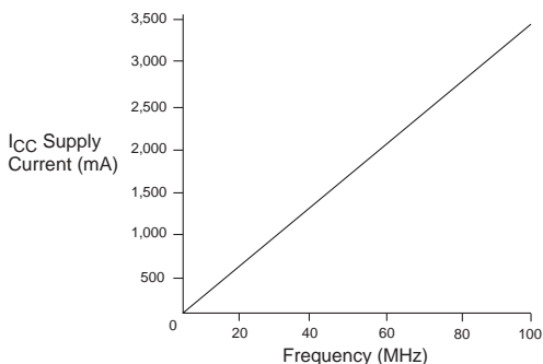
Figure 32. I_{CCACTIVE} vs. Operating Frequency (Part 3 of 3)
