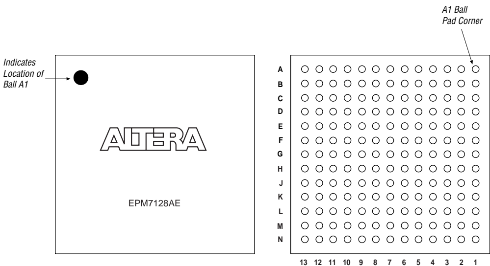
Package outline not drawn to scale.
