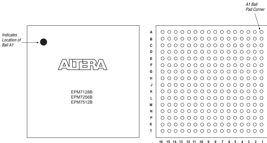
Package outline not drawn to scale.
