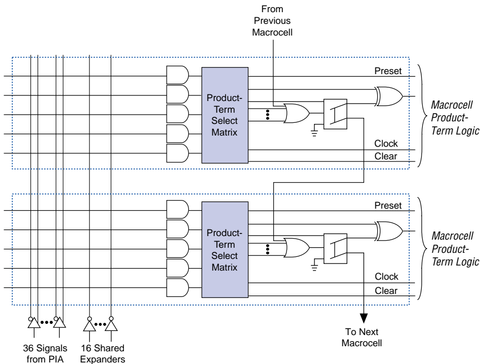
Unused product terms in a macrocell can be allocated to a neighboring macrocell.
