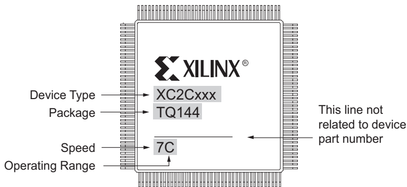
Part Marking for all non chip scale packages
