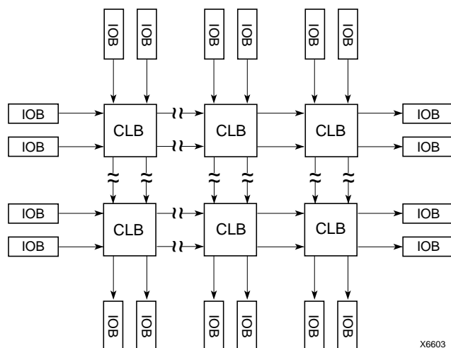
Figure 30: XC4000X Direct Interconnect
