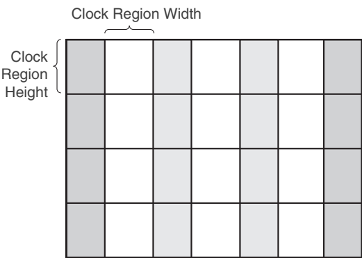
Figure 2: Column-Based FPGA Divided into Clock Regions
